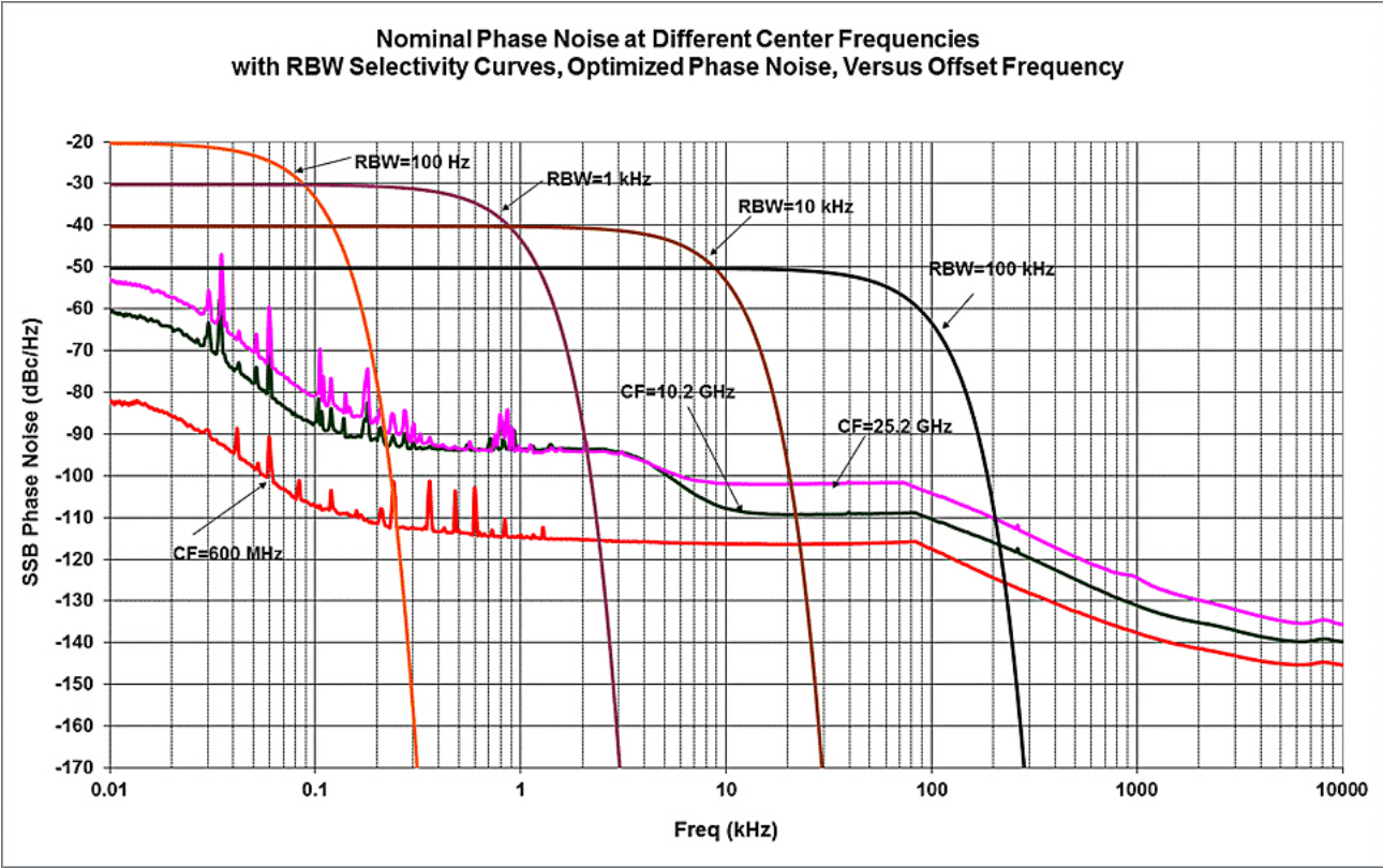
Figure 3. Nominal phase noise at different center frequencies (Applies for instruments with SN prefix ≥ MY/SG/US5233; ships standard with N9020A-EP2)
