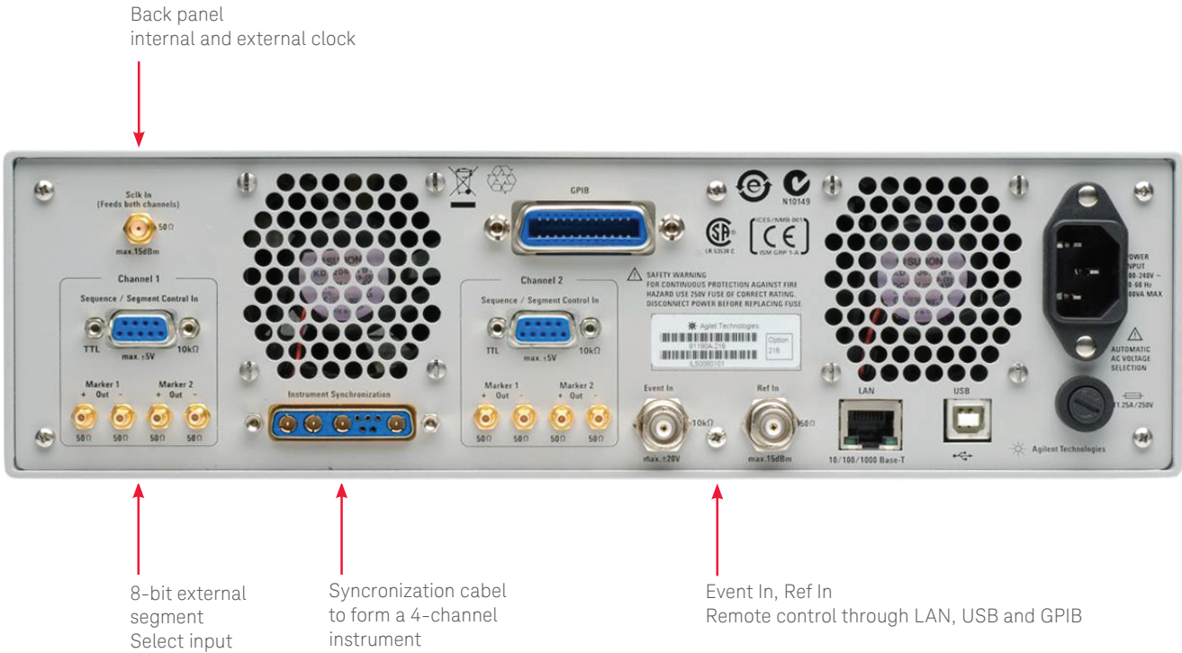
Figure 3. Back panel
