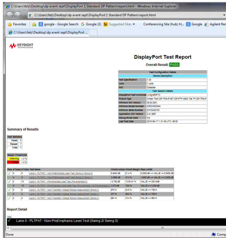
Figure 10. The DisplayPort compliance software generates a summary report where you can see the total test results for your device quickly and clearly. Additional details are available for each test, including the test limits, test description, and test results, including waveforms, if appropriate. All are hot linked to more detailed results further in report. In addition, the margin of the result is indicated to provide further insight.
