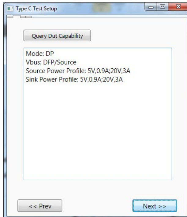
Figure 14. Type-C Setup: Device is queried for PDO capability.
