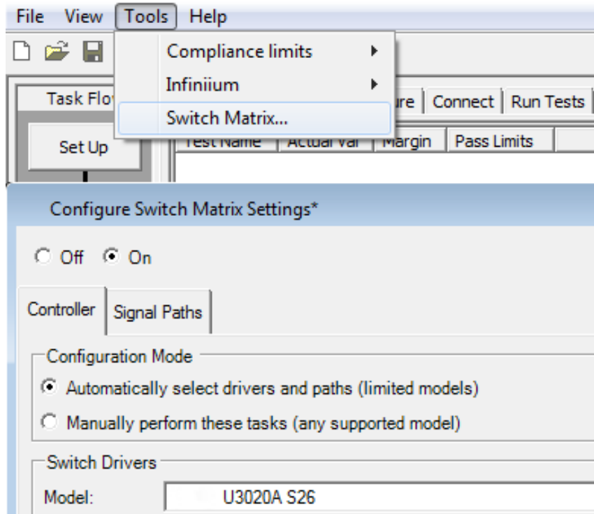
Figure 21. Switch matrix software feature enabled in the compliance application.
