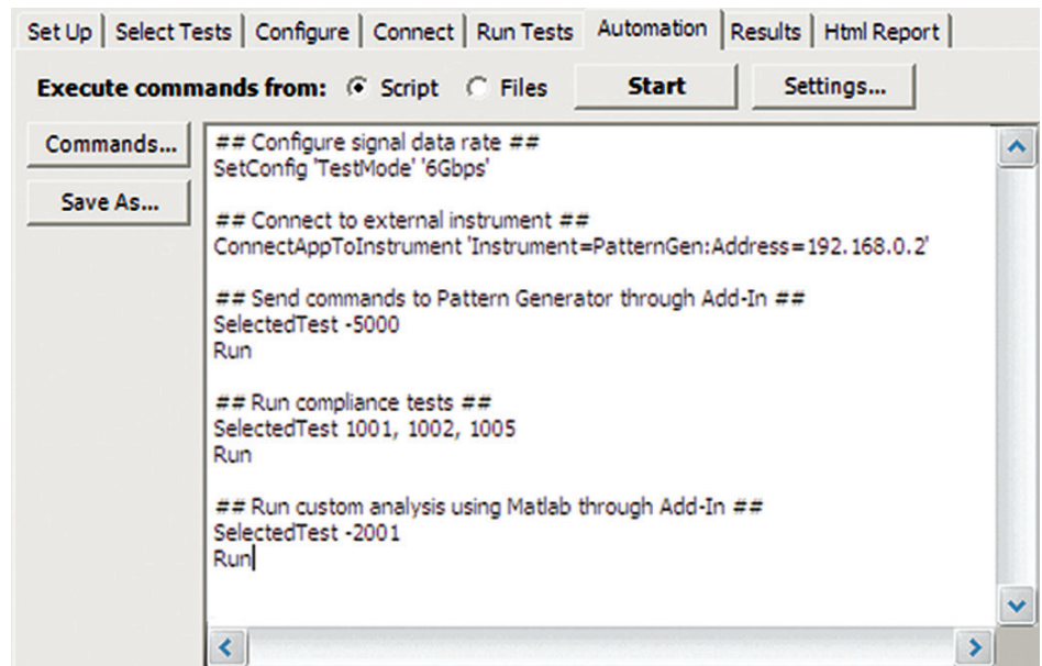
Figure 18. Remote Programming script in the Automation tab.
