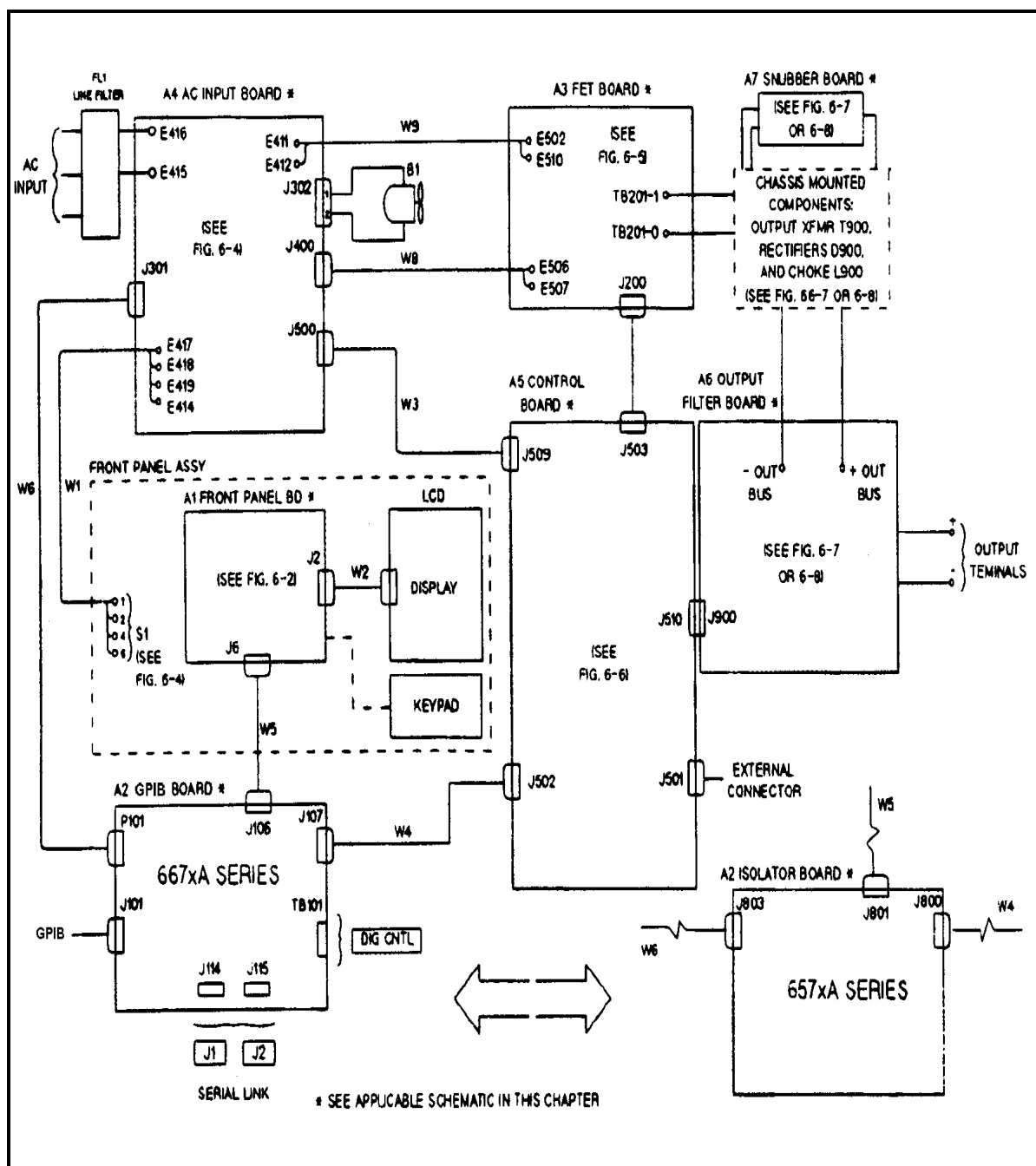
Figure 6-2. Circuit Board Cabling Diagram
