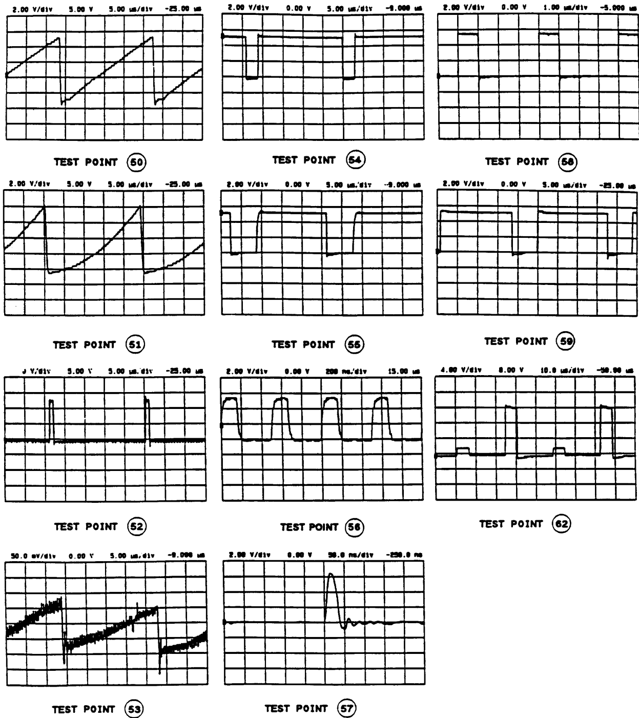
Figure 6-1. Test Point Waveforms for Table 6-3
