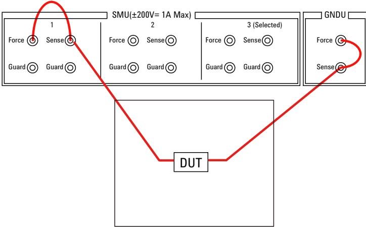
4-wire connections
