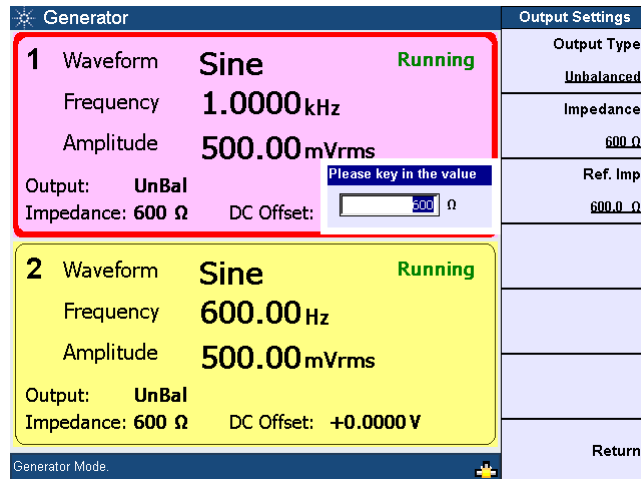
Figure 3-18 Reference impedance
