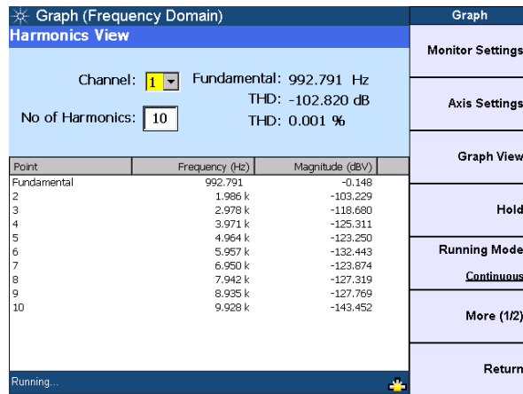
Figure 6-6 Harmonics display
