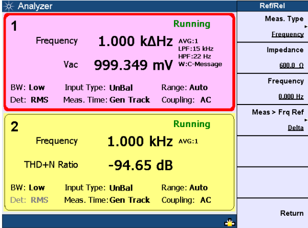
Figure 3-15 Reference Frequency
