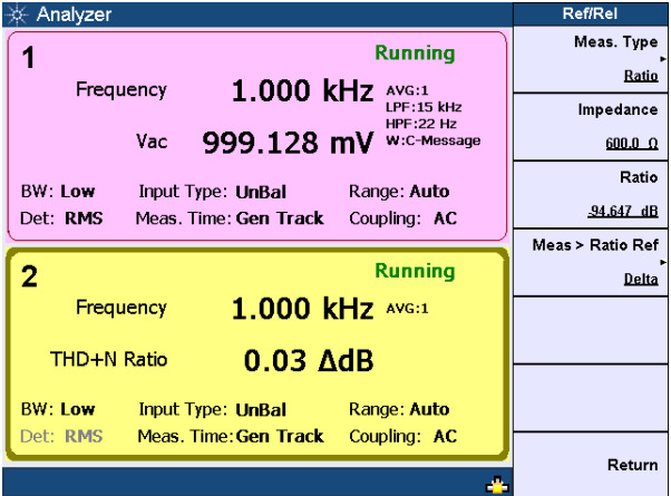
Figure 3-16 Reference Ratio
