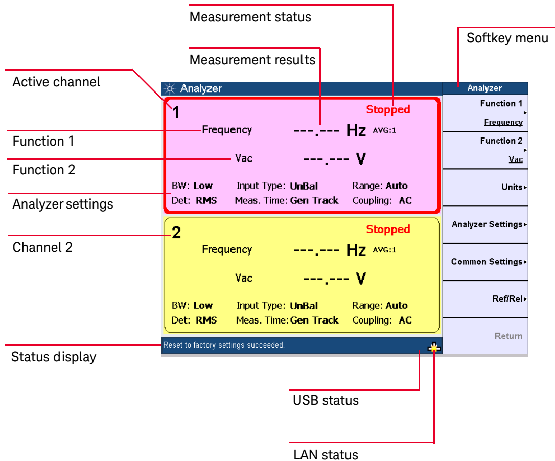
Figure 1-3 Power-up display
