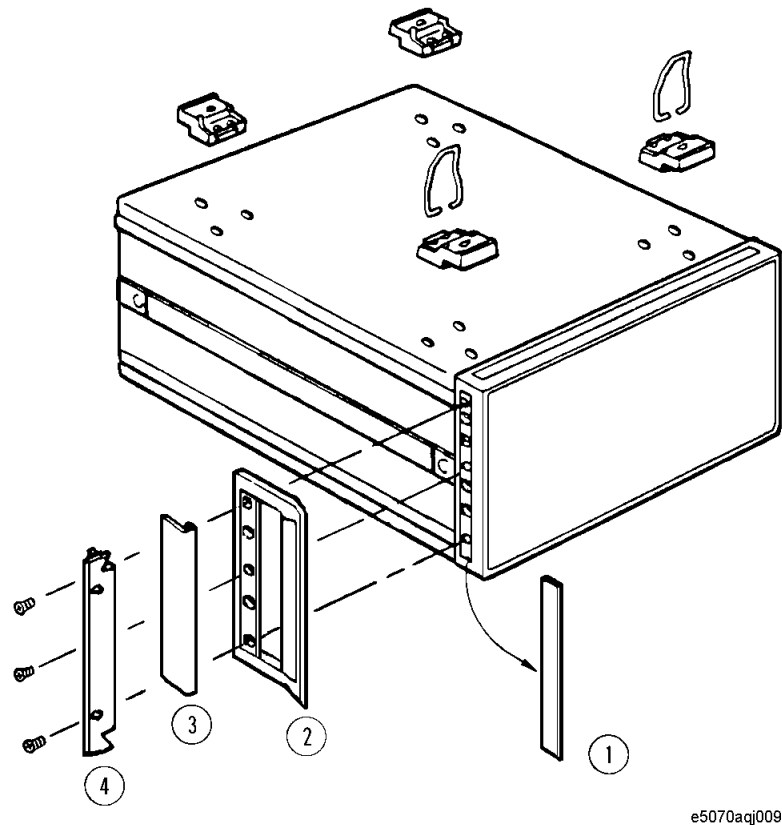
Figure 1-3 Installing front handle/rack-mount kits
