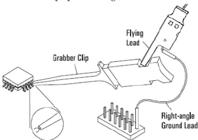
Figure 63 Grabber configuration
