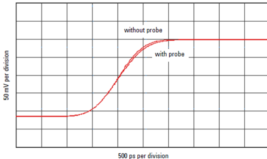
Figure 34 TDT measurement at receiver with and without probe load for 1 ns rise time
