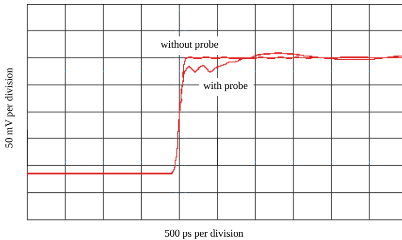
Figure 67 TDT measurement at receiver with and without probe load for 100 ps rise time
