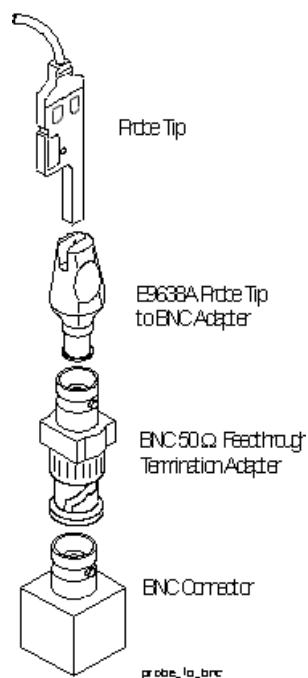
Figure 81 BNC connector
