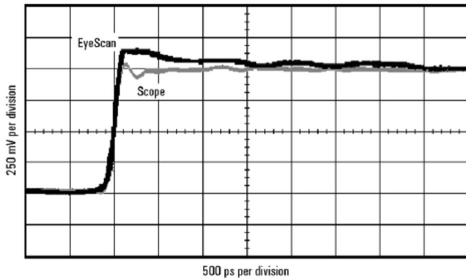
Figure 18 Logic analyzer's response to a 250 ps rise time
