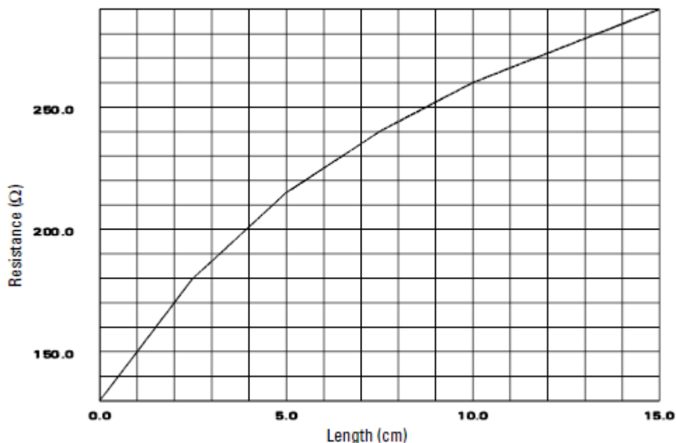
Figure 29 Optimum Damping Resistor Value Versus Signal Lead Length
