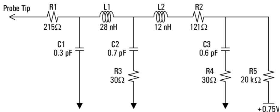
Figure 27 Equivalent load model
