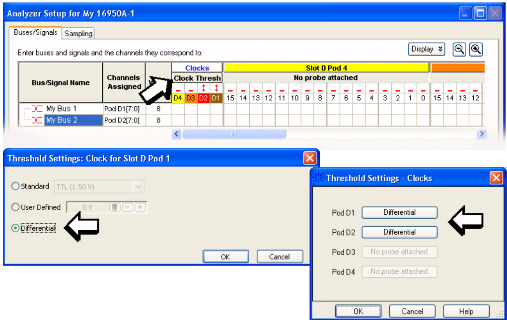
Figure 6 Differential threshold
