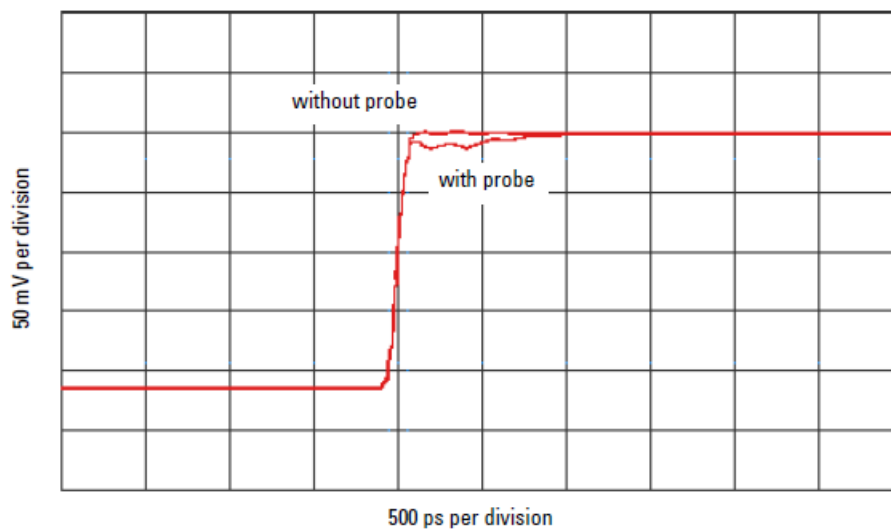
Figure 31 TDT measurement at receiver with and without probe load for 100 ps rise time
