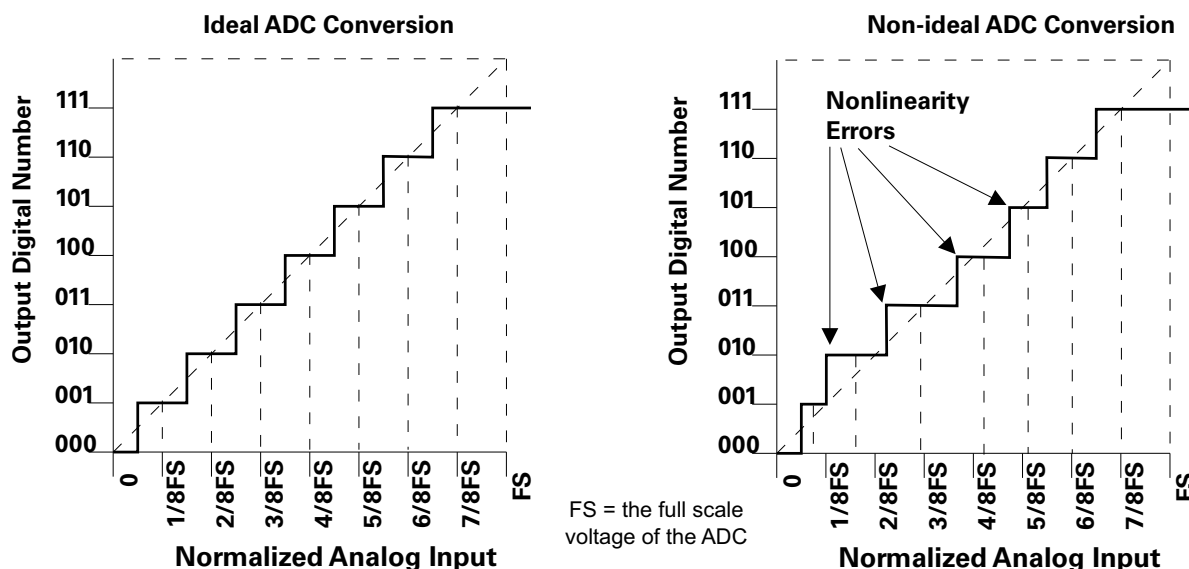
Figure 8 ADC Non-linearity Errors for a 3-bit ADC
