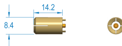
300 V PCB Adapter
