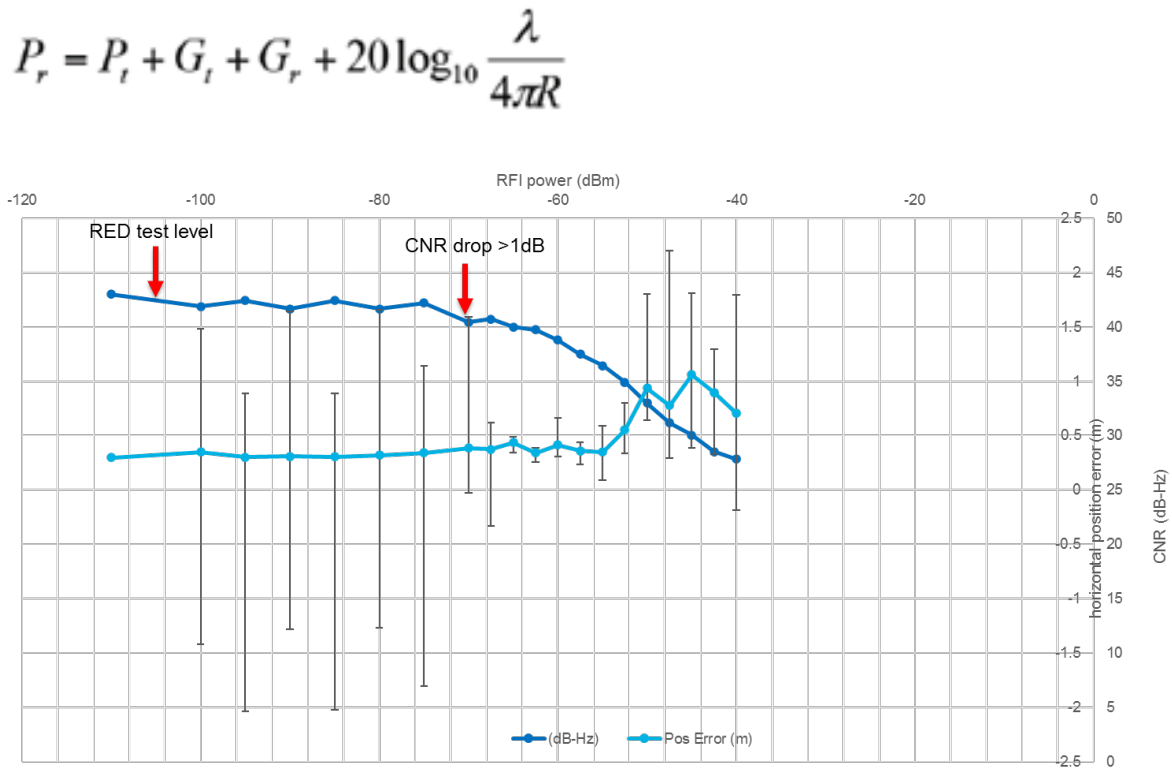
RFI Power and Horizontal position error at 1554MHz with measurement range (HPE) added - Receiver A
