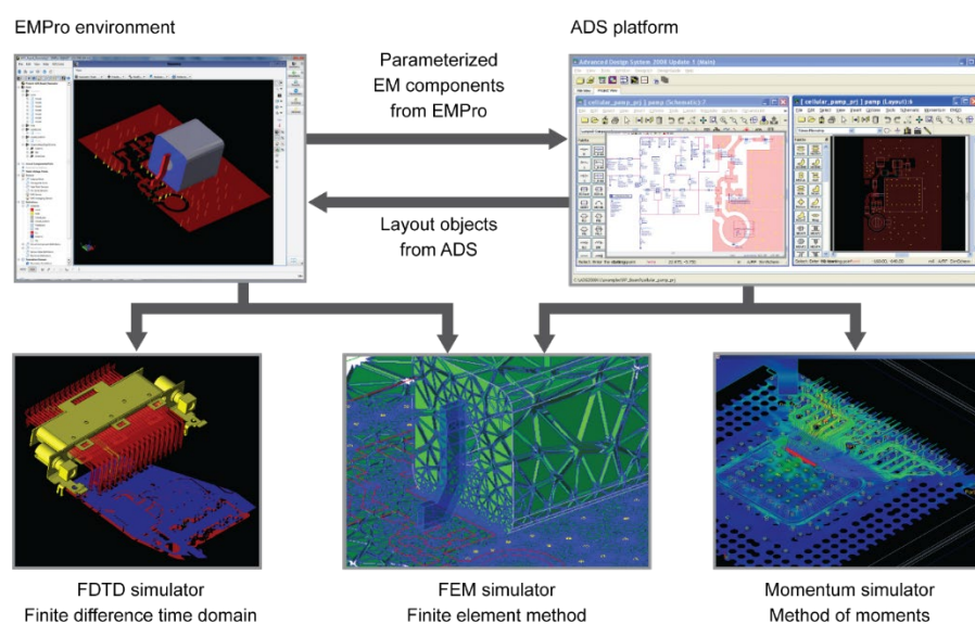
Figure 1. Keysight provides multiple EM simulation technologies integrated with the ADS design flow.
