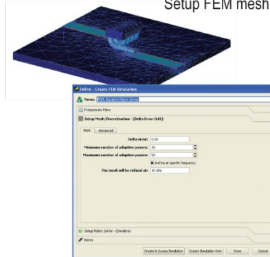
Setup FEM mesh
