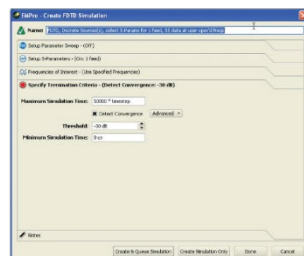
FDTD
