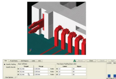
Setup FDTD grid/mesh
