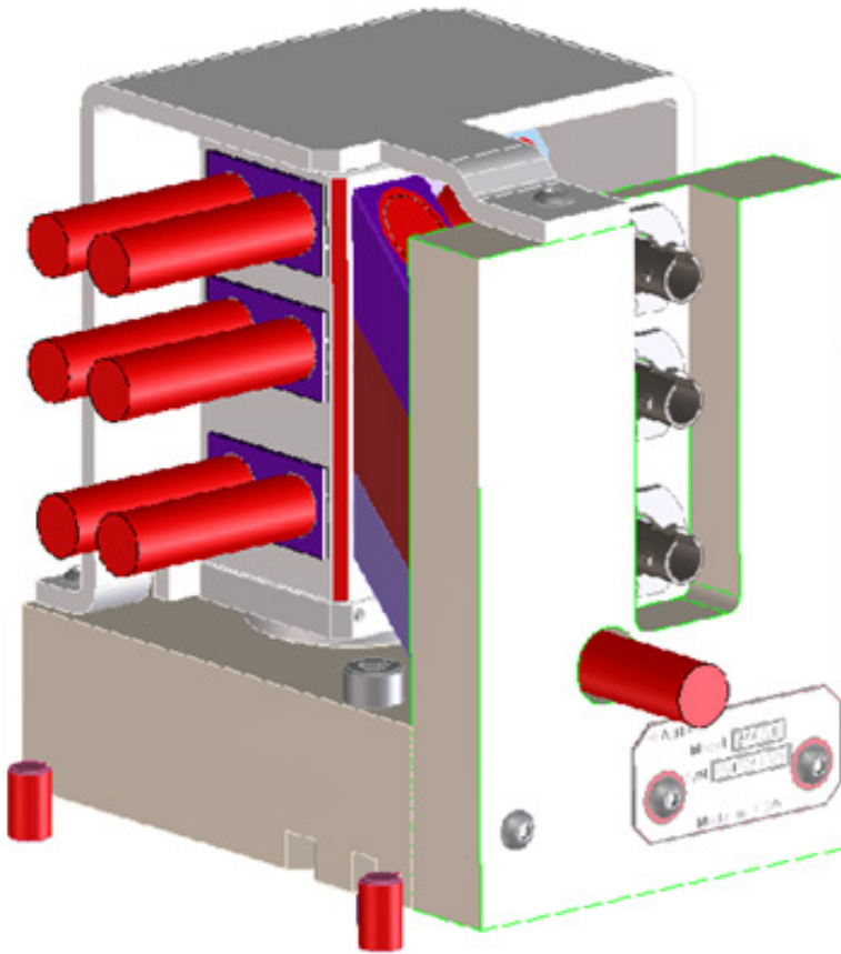
Z4422B Three-Axis Plane Mirror Interferometer showing one face positioned against 2 of the 3 customer supplied datum pins.
