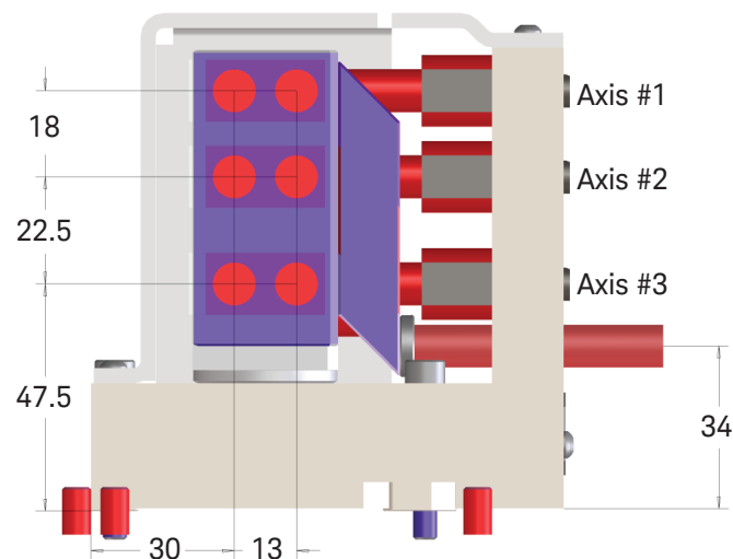
Z4422B beam position in mm and axis numbering
