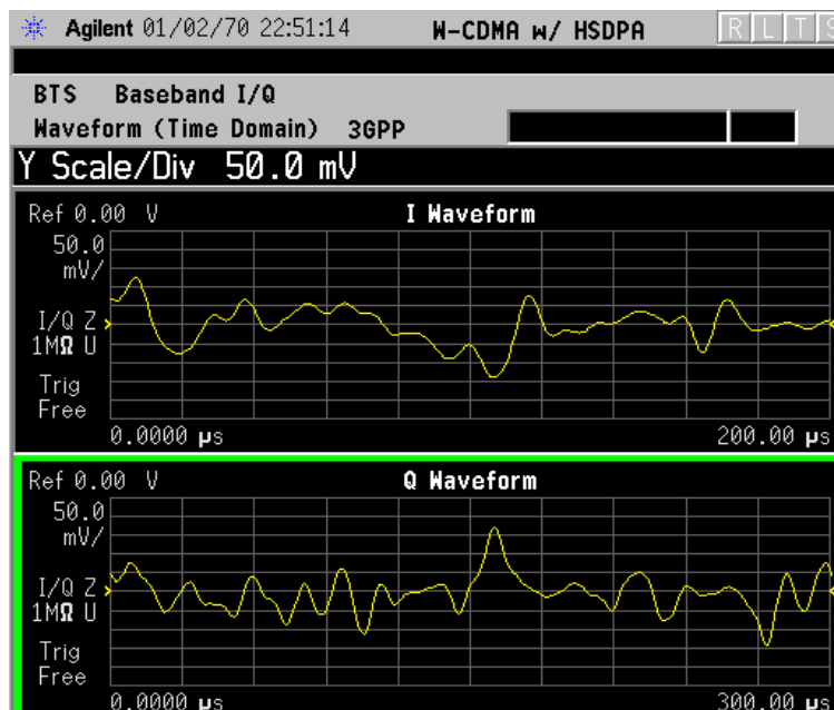
Figure 2-74 Waveform Measurement - I and Q Waveform View
