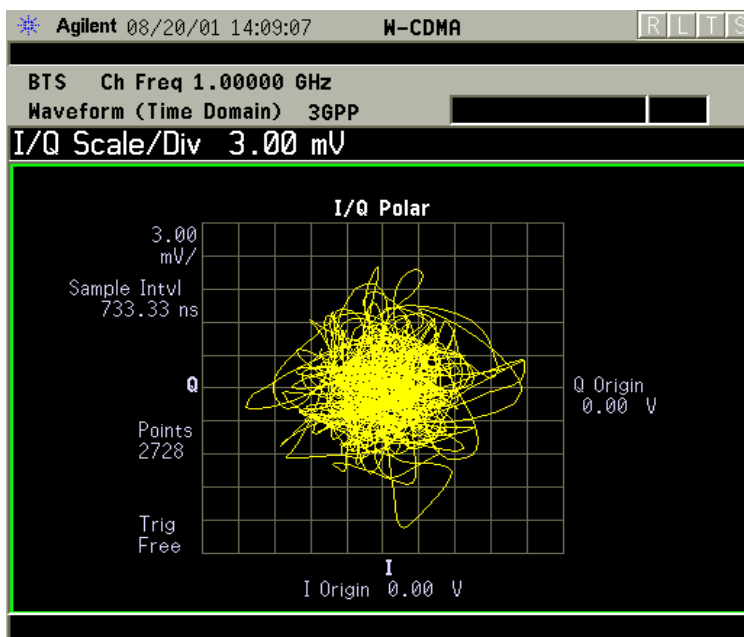
Figure 2-78 Waveform Measurement - I/Q Polar View
