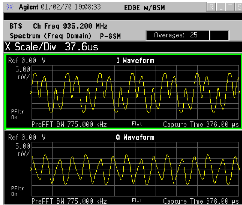
Figure 3-32 Spectrum Measurement - I and Q Waveform View (for E4406A)
