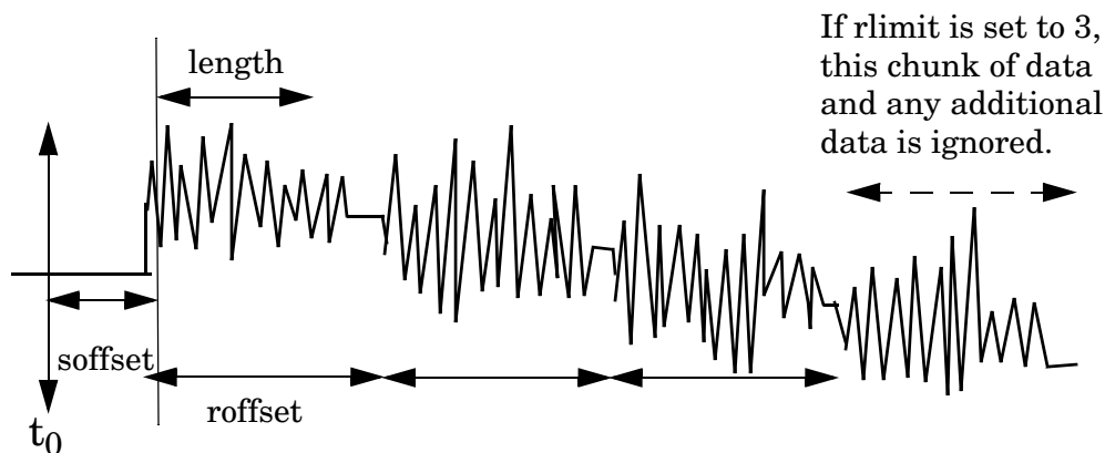
Figure 4-2 Sample Trace Data - Not Constant Envelope
