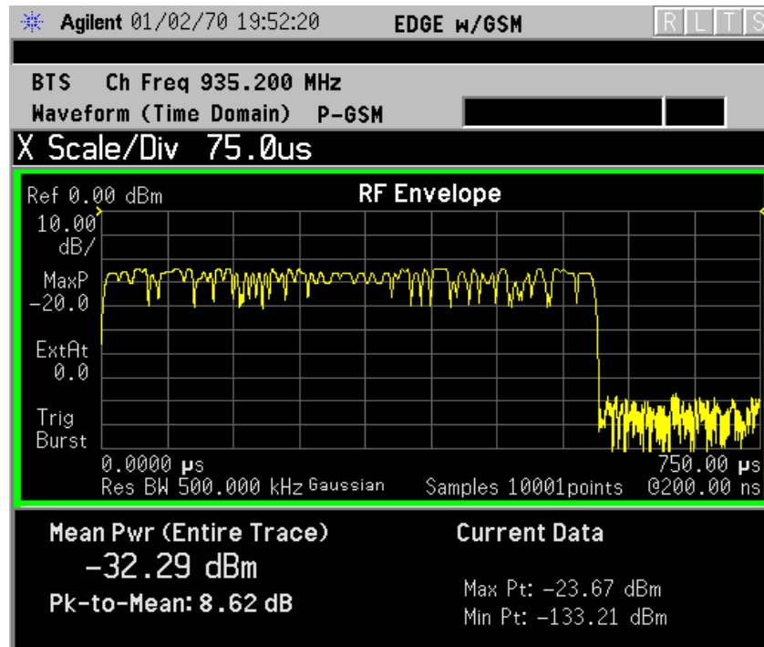
Figure 3-37 Waveform Measurement - RF Envelope (Default View)
