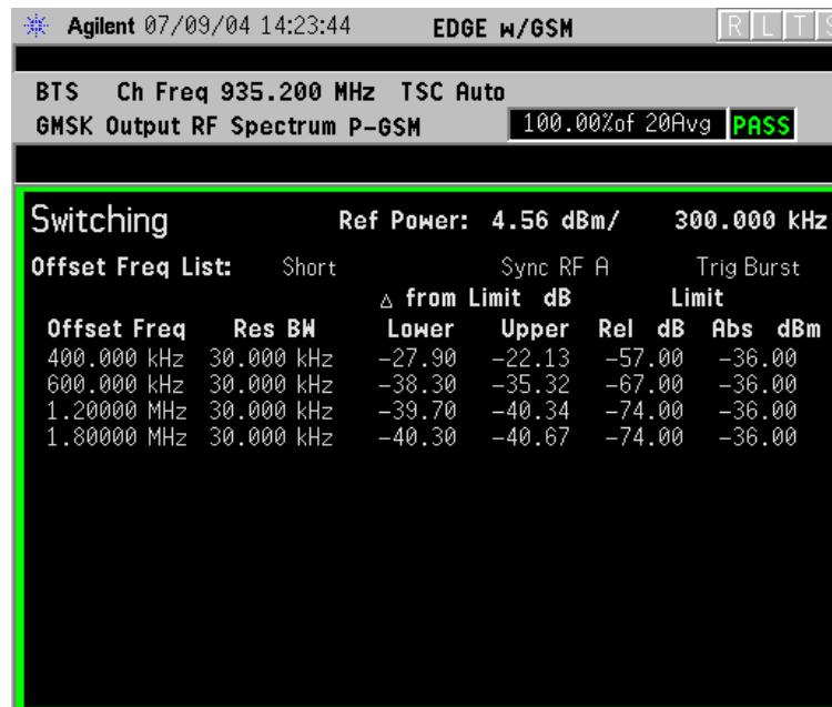
Figure 2-26 GMSK ORFS Result - Switching Margin & Limits View
