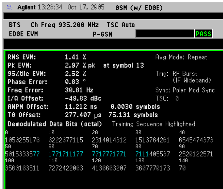
Figure 2-9 EDGE EVM Result - Data Bits View
