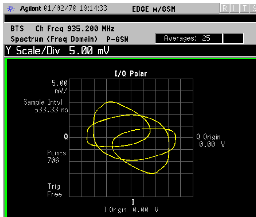
Figure 3-34 Spectrum Measurement - I/Q Polar View (for E4406A)
