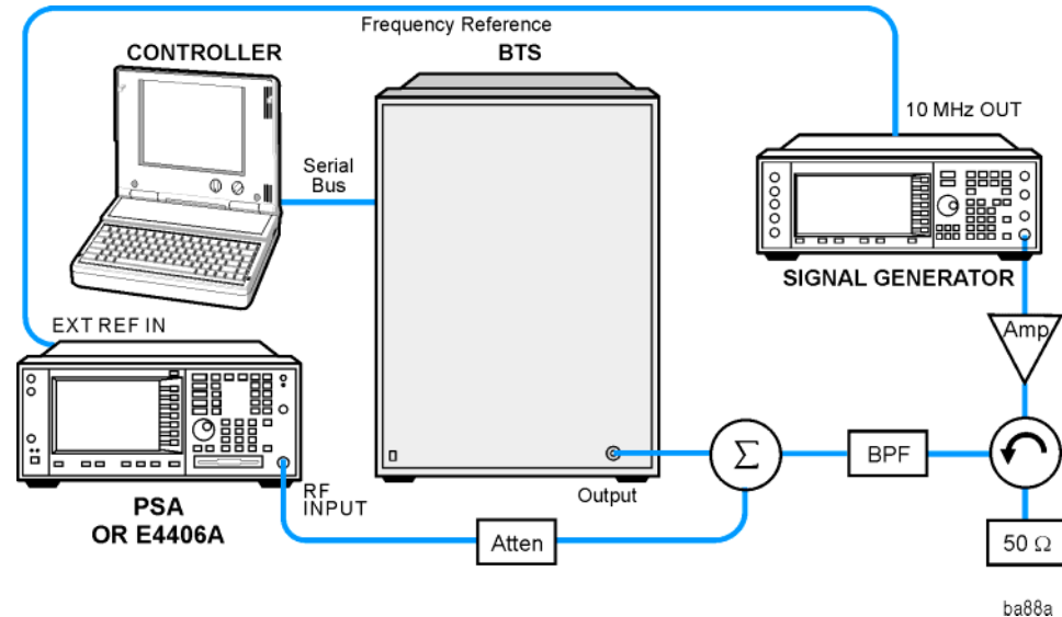
EDGE Transmitter Band Spurious Measurement System
