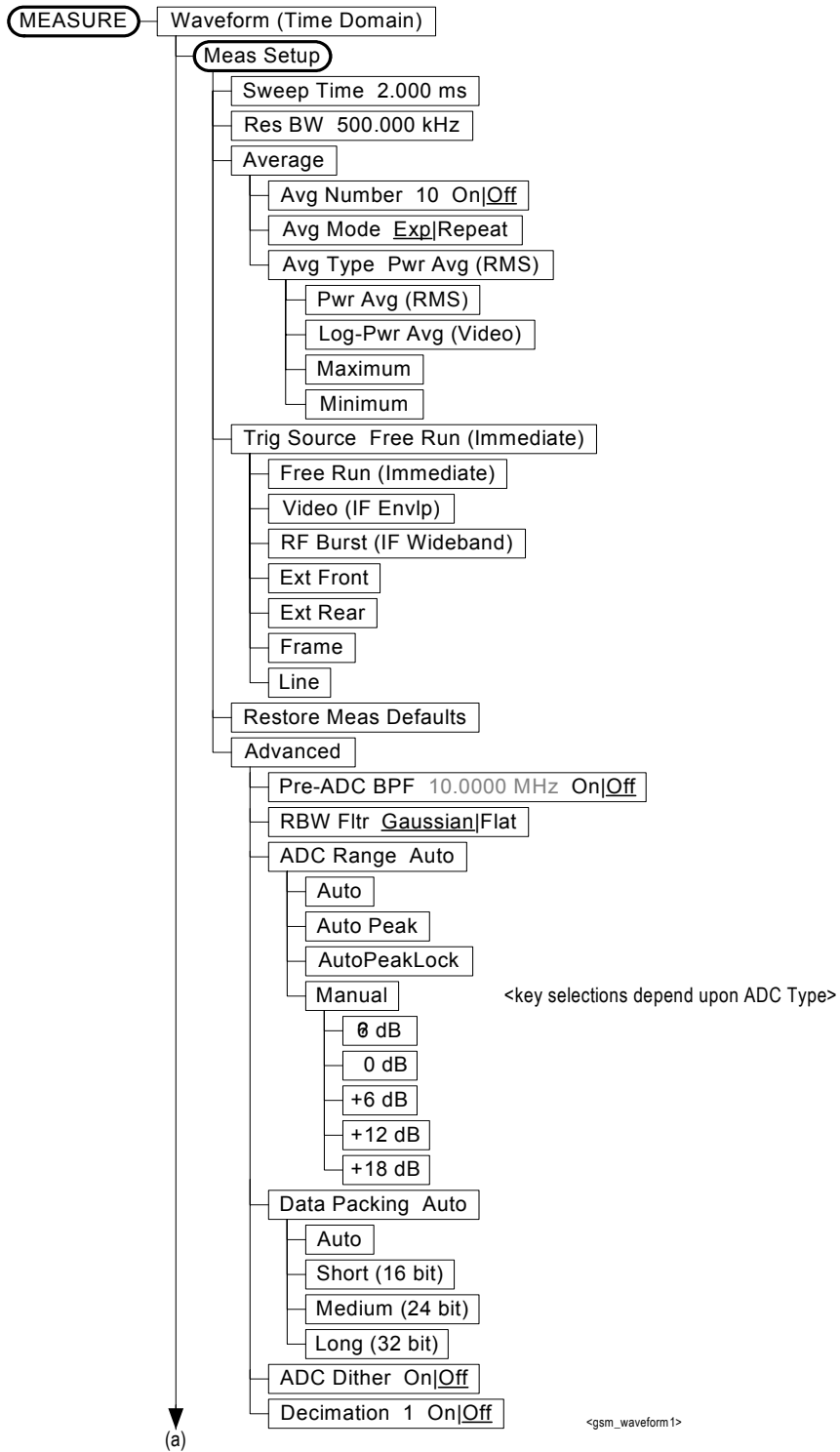
Figure 6-23 Waveform (Time Domain) Measurement Key Flow (1 of 2)
