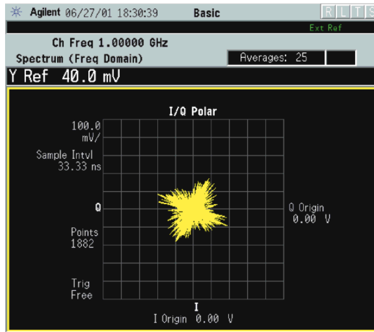
Figure 3-33 Spectrum Measurement - I/Q Polar View (for E4406A)
