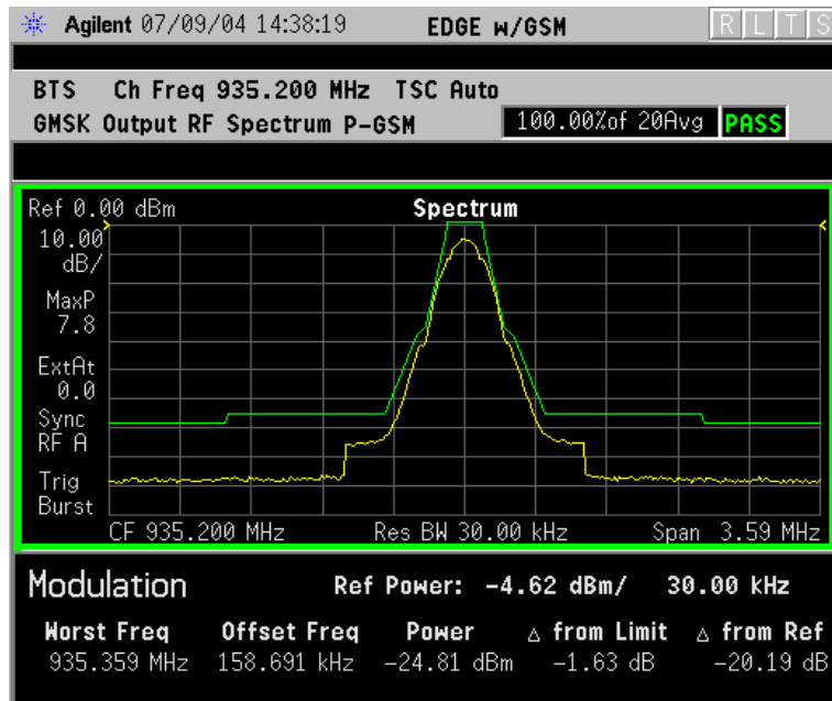
Figure 2-30 GSMK ORFS Result - Example Modulation Swept View
