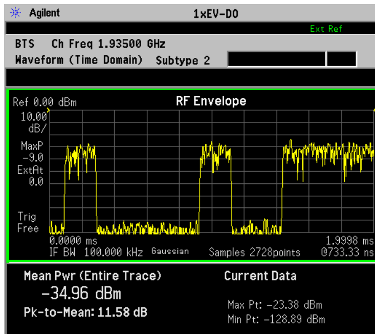
Figure 3-38 Waveform Measurement - RF Envelope (Default View)
