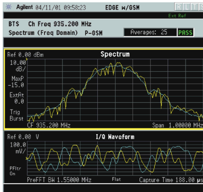
Figure 2-47 Spectrum Measurement - Spectrum and I/Q Waveform (Default) View
