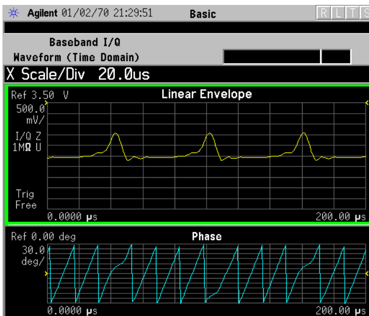
Figure 2-66 Waveform Measurement - Linear Envelope View
