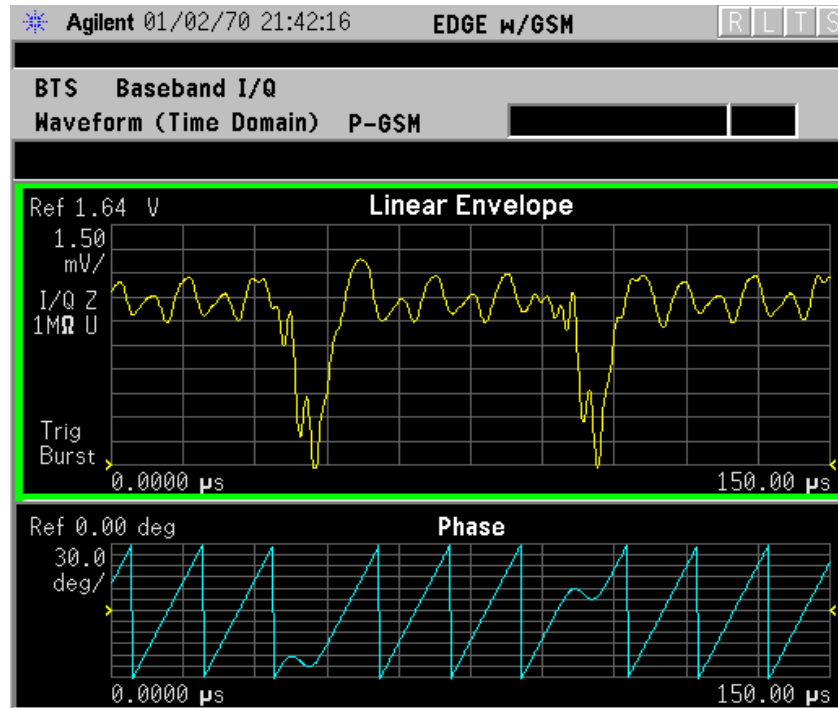
Figure 3-43 Waveform Measurement - I and Q Waveform View
