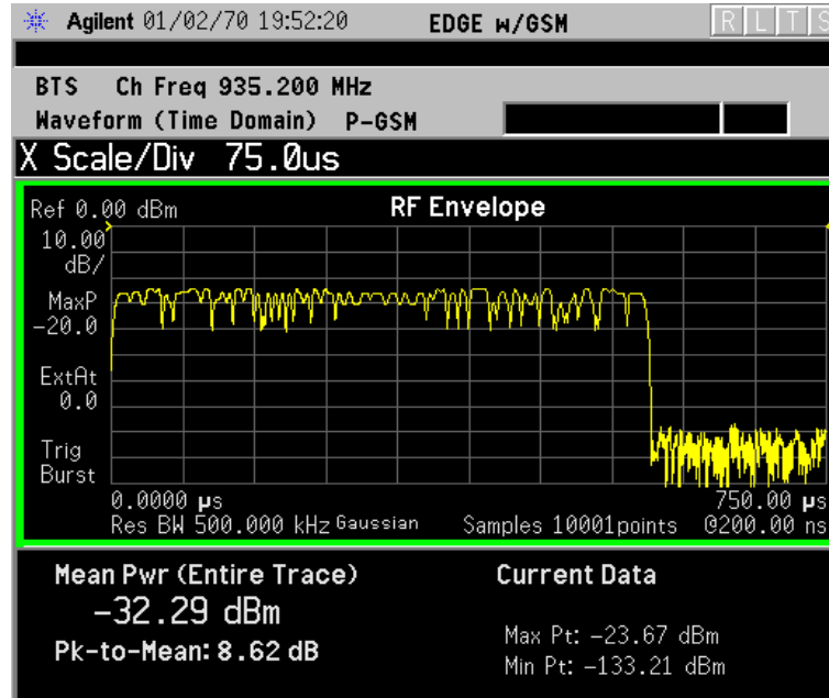
Figure 2-65 Waveform Measurement - RF Envelope (Default View)
