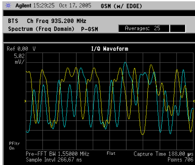
Figure 2-48 Spectrum (Time Domain) Measurement - I/Q Waveform Result
