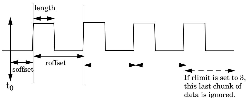
Figure 4-1 Sample Trace Data - Constant Envelope
