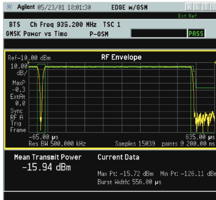
Figure 2-39 GMSK Power vs. Time Result - Burst View
