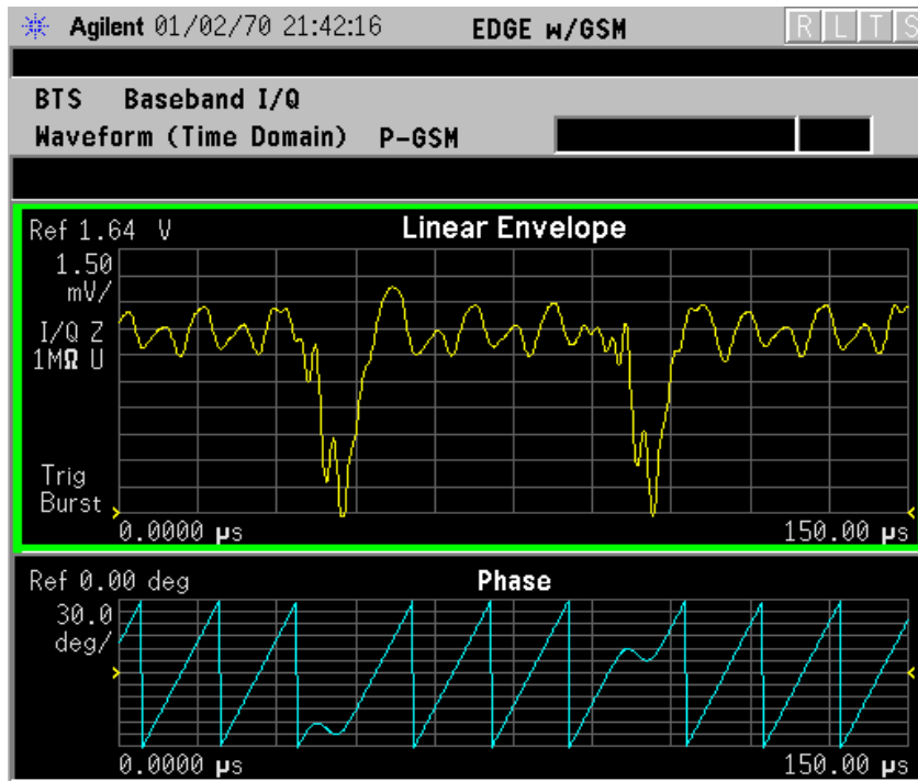
Figure 3-40 Waveform Measurement - Linear Envelope View
