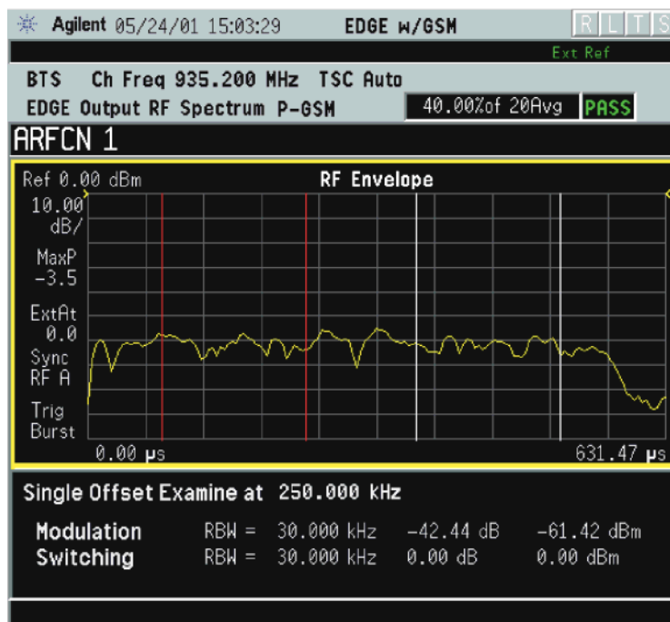
EDGE ORFS Result - Modulation with Single-Offset (Examine)
