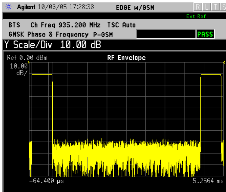
Figure 2-35 GSMK Phase and Frequency Error Result - RF Envelope View
