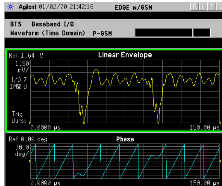
Figure 2-69 Waveform Measurement - Linear Envelope View
