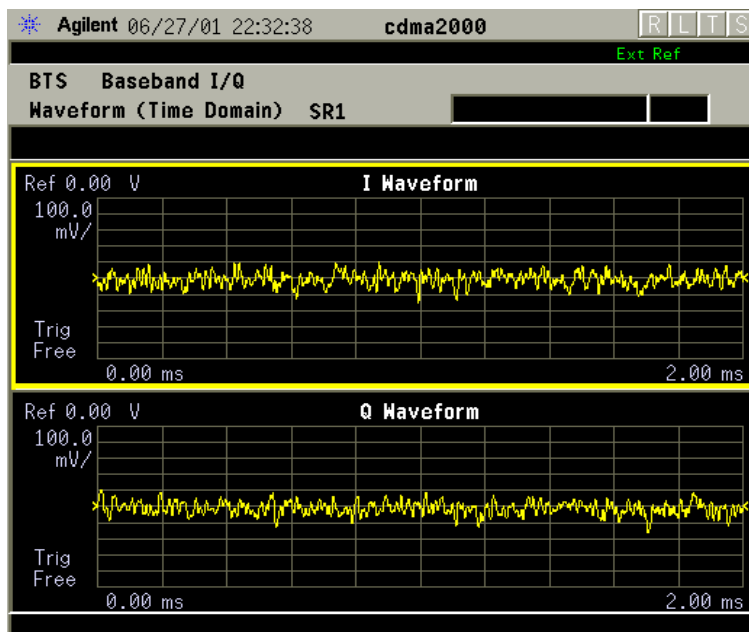
Figure 2-73 Waveform Measurement - I and Q Waveform View
