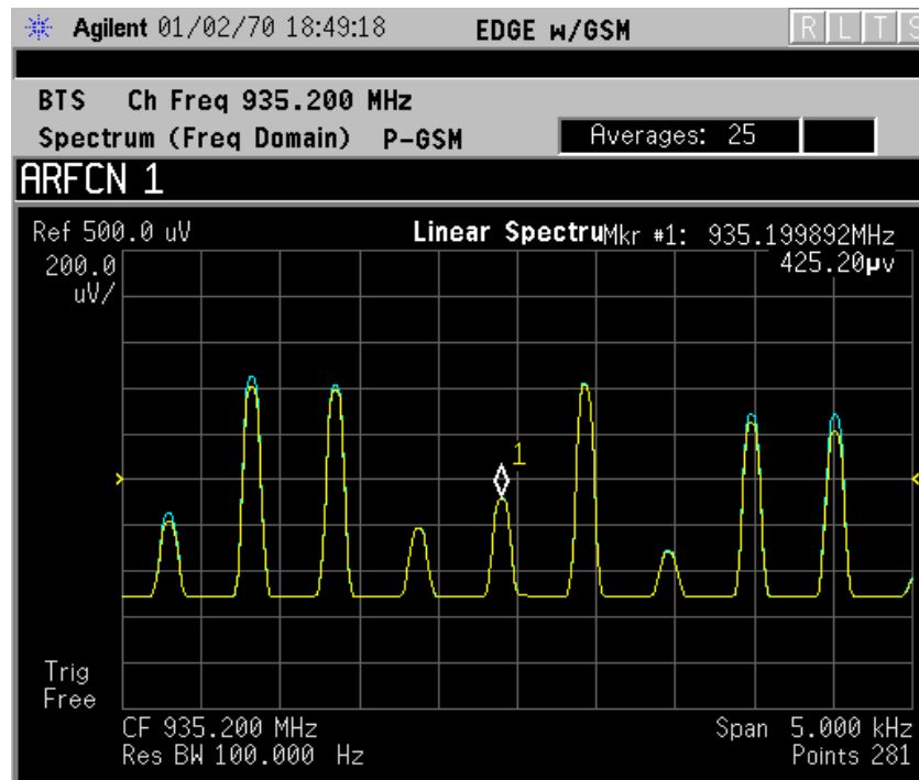
Figure 3-30 Spectrum Measurement - Linear Spectrum View (for E4406A)
