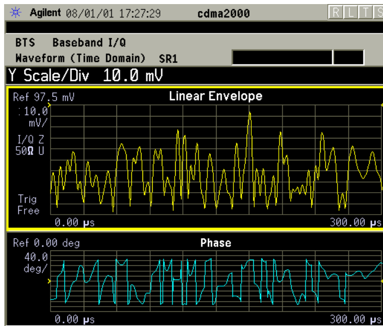
Figure 2-67 Waveform Measurement - Linear Envelope View
