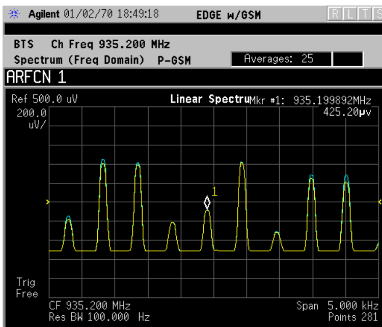
Figure 2-50 Spectrum Measurement - Linear Spectrum View (E4406A)
