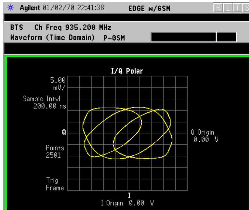
Figure 3-45 Waveform Measurement - I/Q Polar View
