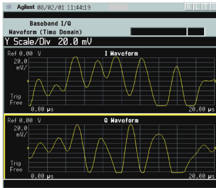
Figure 2-71 Waveform Measurement - I and Q Waveform View
