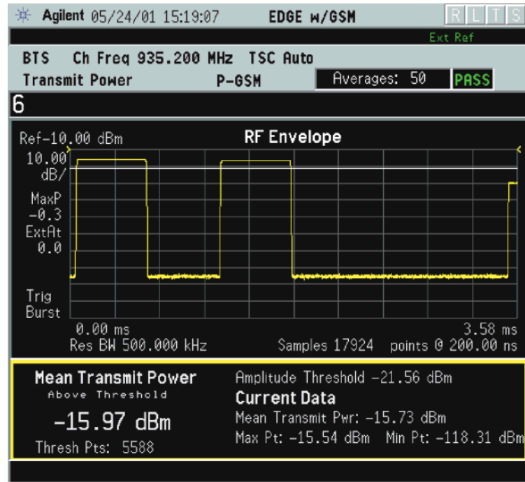
Figure 2-63 Transmit Power Result - Multiple Bursts
