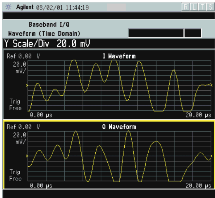
Figure 2-84 I and Q Waveform View - Baseband I/Q Inputs
