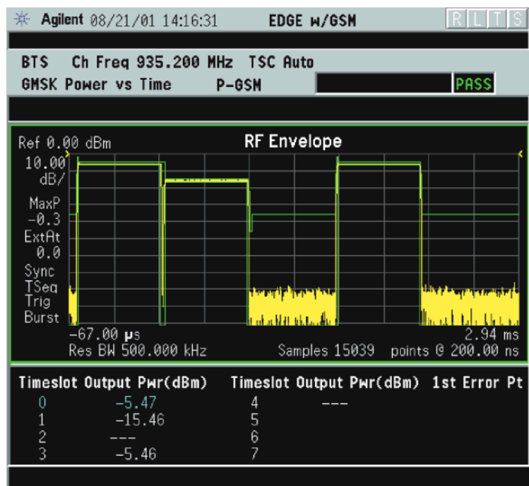
Figure 2-41 GSMK Power vs. Time Result - Multi-Slot View (5 slots shown)
