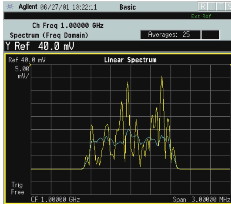
Figure 3-30 Spectrum Measurement - Linear Spectrum View (for E4406A)
