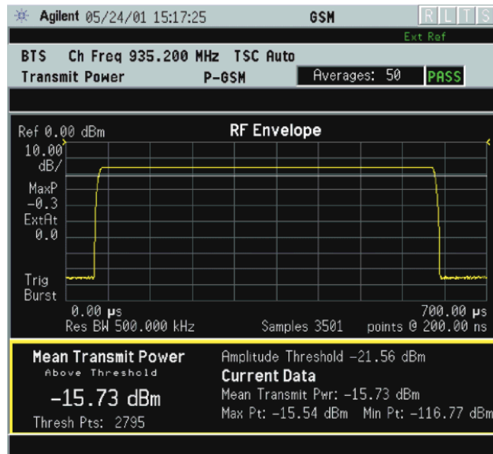
Figure 2-62 Transmit Power Result - Single Burst (with data table)
