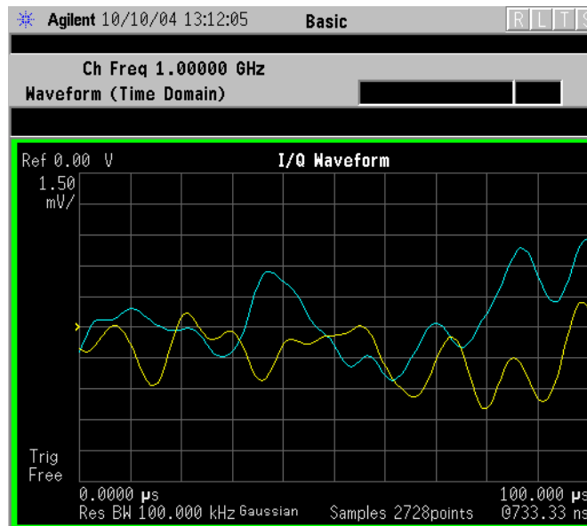
Figure 3-41 Waveform Measurement - I/Q Waveform View
