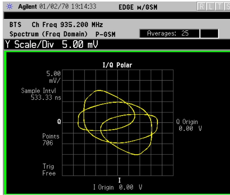
Figure 2-60 Spectrum Measurement - I/Q Polar View (E4406A)
