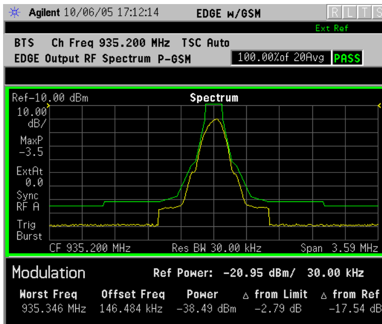
Figure 2-18 EDGE ORFS Result - Example Modulation Swept View
