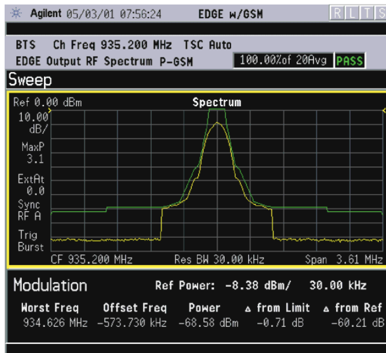
EDGE ORFS Result - Modulation Sweep Spectrum
