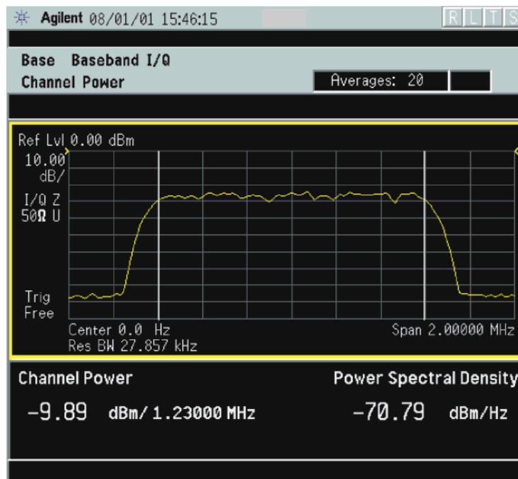
Figure 2-80 Channel Power - Baseband I/Q Inputs
