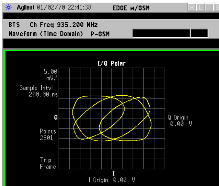
Figure 2-76 Waveform Measurement - I/Q Polar View
