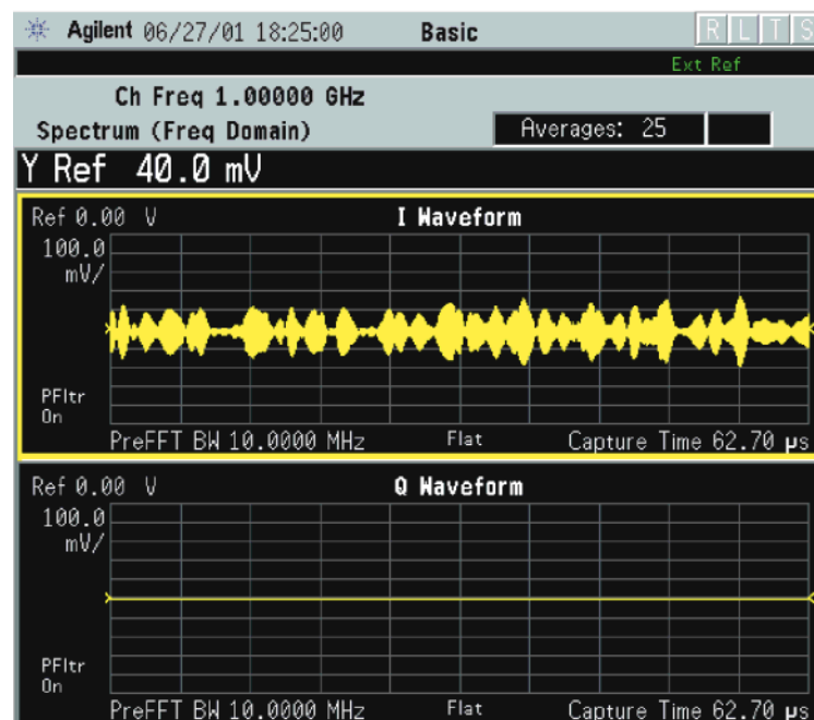
Figure 3-31 Spectrum Measurement - I and Q Waveform View (for E4406A)
