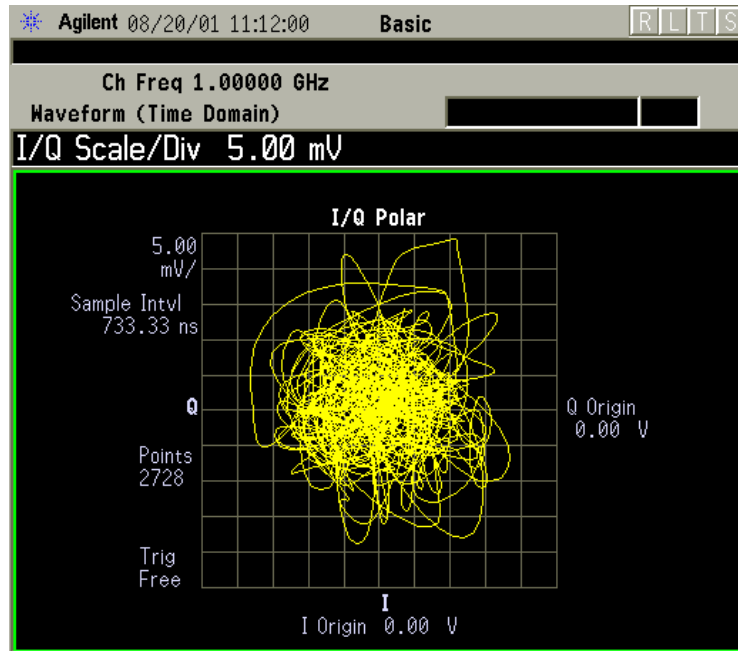
Figure 3-45 Waveform Measurement - I/Q Polar View
