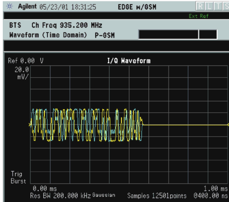
Figure 3-42 Waveform Measurement - I/Q Waveform View
