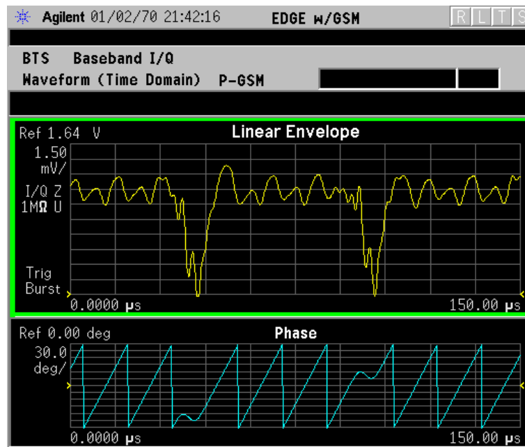
Figure 2-72 Waveform Measurement - I and Q Waveform View
