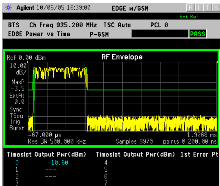
Figure 2-4 EDGE Result - Multi-Slot View
