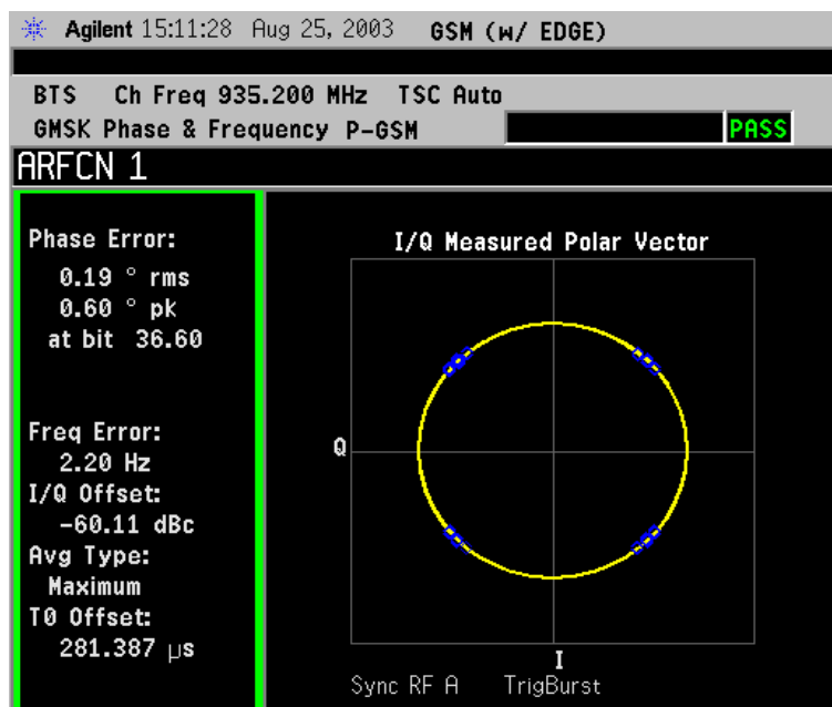
Figure 2-36 GSMK Phase and Frequency Error Result - Polar View
