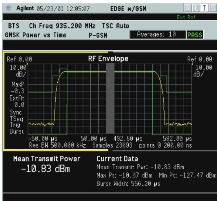
Figure 2-40 GSMK Power vs. Time Result - Rise & Fall View
