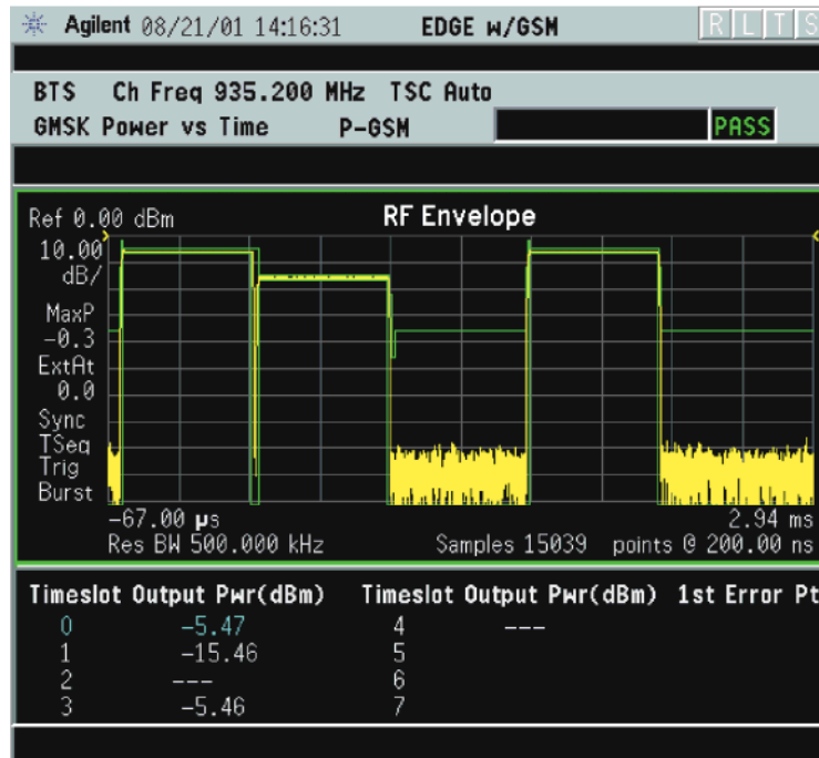
Figure 3-25 GSMK Power vs. Time Result - Multi-Slot View (5 slots shown)
