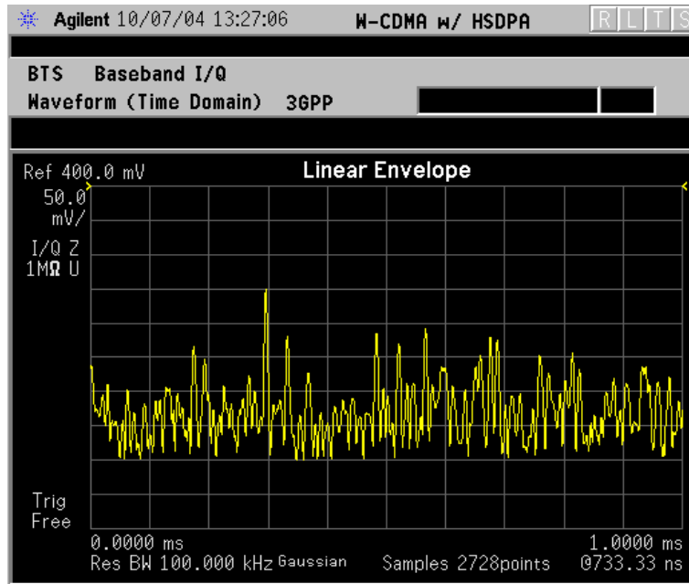
Figure 2-68 Waveform Measurement - Linear Envelope View
