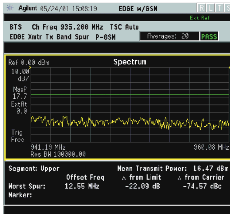
Figure 3-26 EDGE Tx Band Spur Result - Upper Adj Segment
