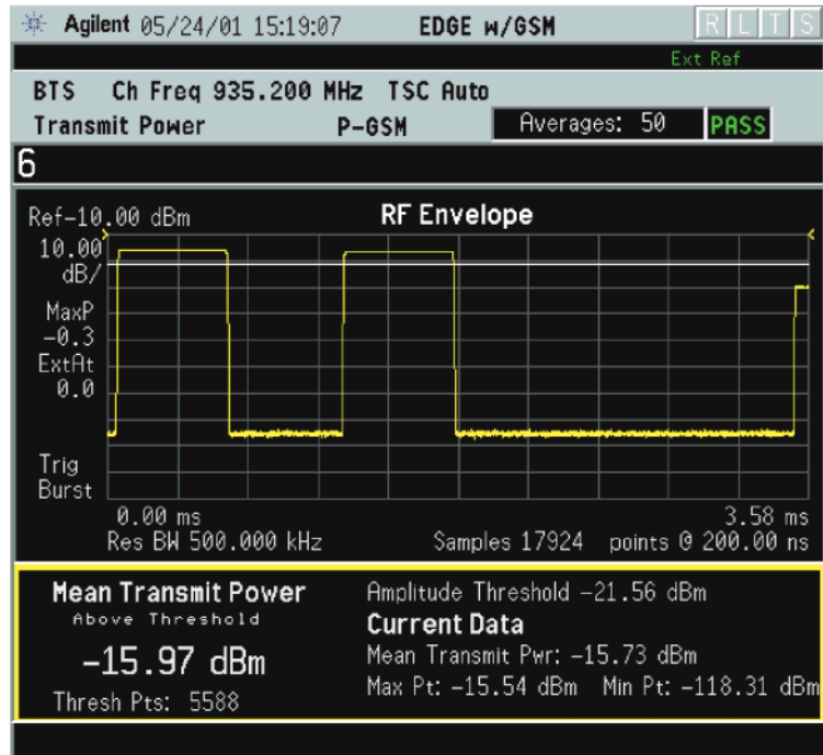
Figure 3-36 Transmit Power Result - Multiple Bursts
