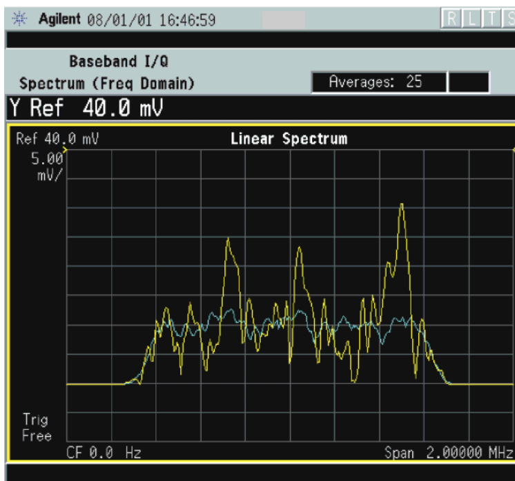
Figure 2-82 Spectrum Linear View- Baseband I/Q Inputs
