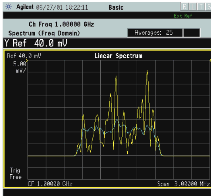
Figure 2-49 Spectrum Measurement - Linear Spectrum View (for E4406A)
